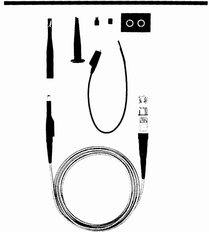
Figure 14. PROBES CONNECT THE SCOPE AND THE CIRCUIT-UNDER-TEST. Tektronix probes consist of a patented resistive cable and a grounded shield. Two P6122 probes and the accessories pictured above are supplied with every 2200 Series scope. The probe is a high impedance, minimum loading 10 X passive probe. The accessories for each probe (from left to right) are: a grabber tip for ICs and small diameter leads; a retractable hook tip; and IC tester tip cover; an insulating ground cover; marker bands; and (in the center) the ground lead.
