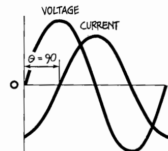
Figure 22. PHASE is best explained with a sine wave. Remember that this waveform is based on the sine of all the angles from 0 through 360. The result is a plot that changes from 0 to 0°, 1 at 90°, 0 again at 180°, -1 at 270°, and finally 0 again at 360°. Consequently, it is useful to refer to the phase angle (or simply phase , when there is no ambiguity) of a sine wave when you want to describe how much of the period has elapsed. Another use of phase is found when you want to describe a relationship between two signals. Picture two clocks with their second hands sweeping the dial every 60 seconds. If the second hands touch the twelve at the same time, the clocks are in phase ; if they don't, then they're out of phase . To express how far out of phase they are, you use phase shift in degrees. To illustrate, the waveform labeled CURRENT in the drawing above is said to be 90° out of phase with the voltage waveform. Other ways of reporting the same information are "the current waveform has a 90 degree phase angle with respect to the voltage waveform" or "the current waveform lags the voltage waveform by 90°." Note that there is always a reference to another waveform; in this case, between the voltage and current waveforms of an inductor.
