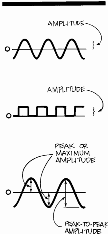
Figure 17. AMPLITUDE IS A CHARACTERISTIC OF ALL WAVEFORMS. It is the amount of displacement from equilibrium at a particular point in time. Note that without a modifier, the word means the maximum change from a reference without regard to the direction of the change. In the first two drawings above (sine wave and square wave), the amplitude is the same even though the sine wave is larger from peak to peak. In the third drawing, an alternating current waveform is shown with peak (or maximum) amplitude and peak-to-peak amplitude parameters annotated. In oscilloscope measurements, amplitude usually means peak-to-peak amplitude.
