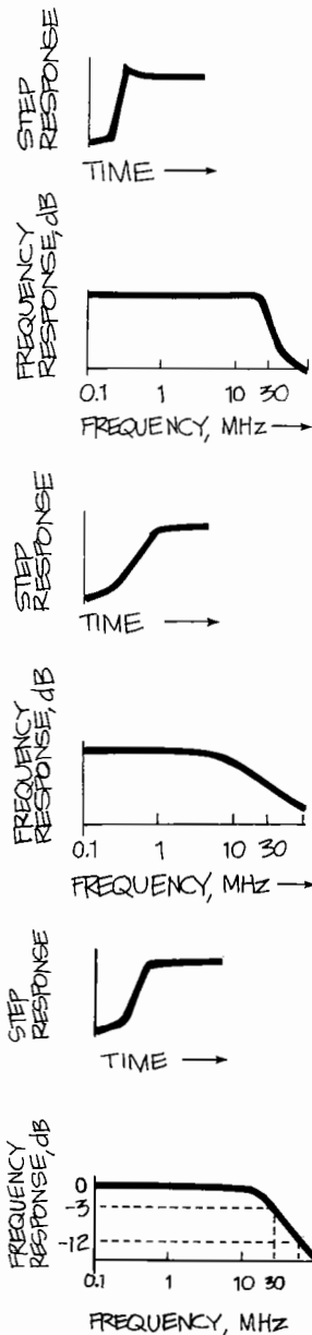
Figure 32. HIGH FREQUENCY COMPENSATION in a scope's vertical amplifier has an effect on the rise time of square waves measured by the scope. If too much high frequency compensation is present, the rise times will show overshoot and possible ringing, as in the top drawing. Too little, as shown in the second drawing, tends to rolloff the edges of the square wave. A critically damped frequency response is best as in the third drawing.
