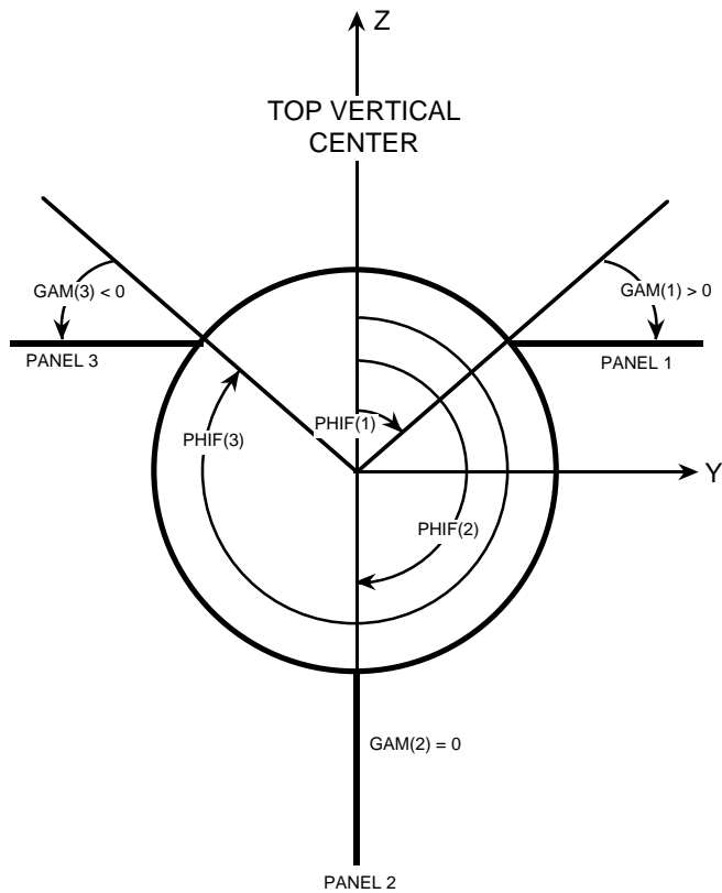
VIEW LOOKING FORWARD FROM BEHIND MISSILE
