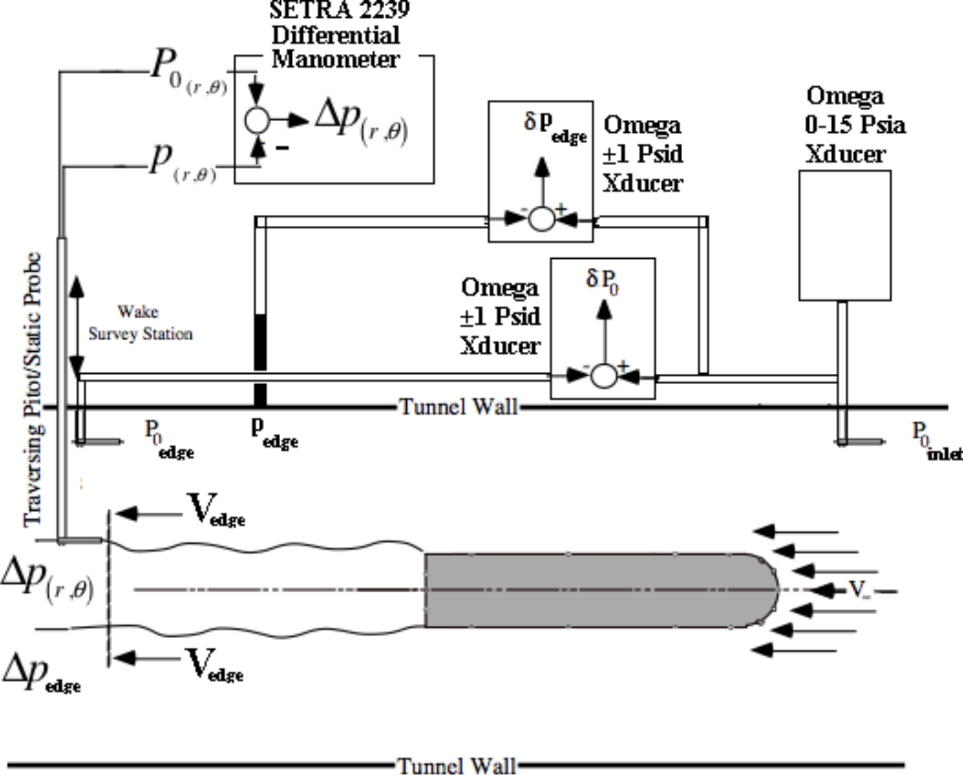
Schematic of Wake Survey Measurements
