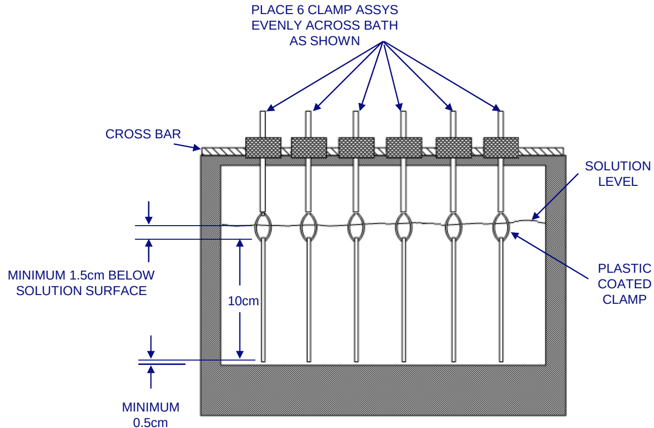
LINDBERG/BUE M WATERBATH MODEL # WB110A SECTION VIEW
